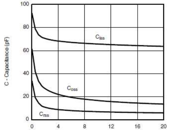
Capacitance
